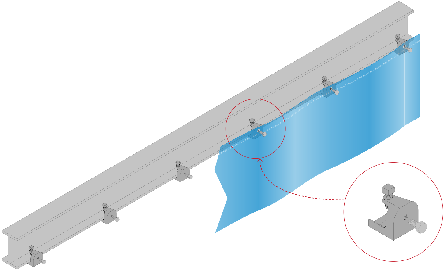
Threaded Rod Clamp (P/N THRCL) 3/8" - 16 Bolt (P/N BLT)
