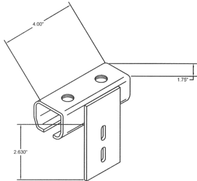
Wall Mount Flange Down Part Number: WMCD-K46
